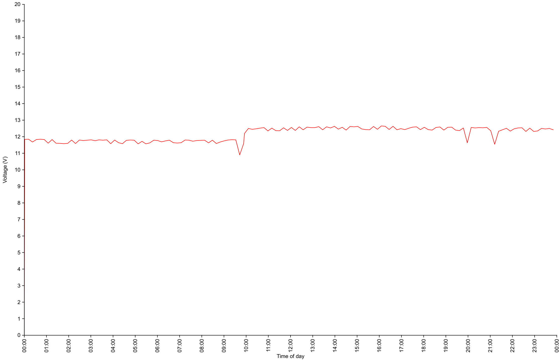
Voltage Daily Overview for Sat Aug 22 2026
