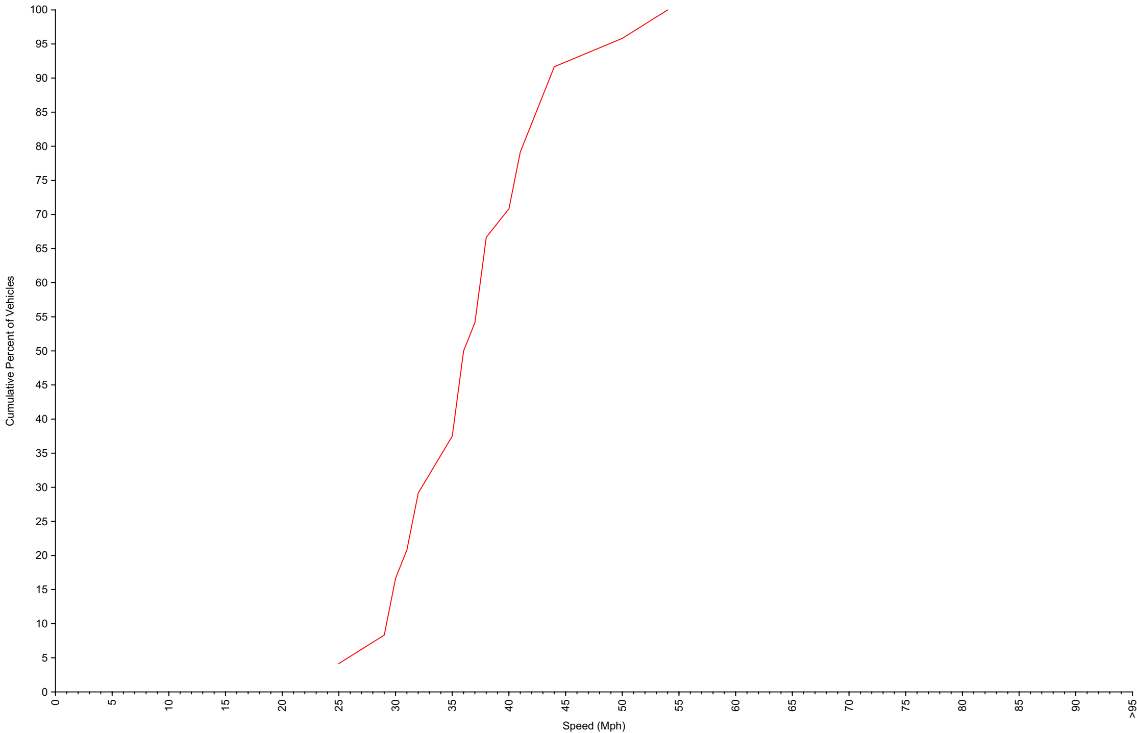
Cumulative Speed Distribution Curve Daily Overview for Mon Aug 31 2026
