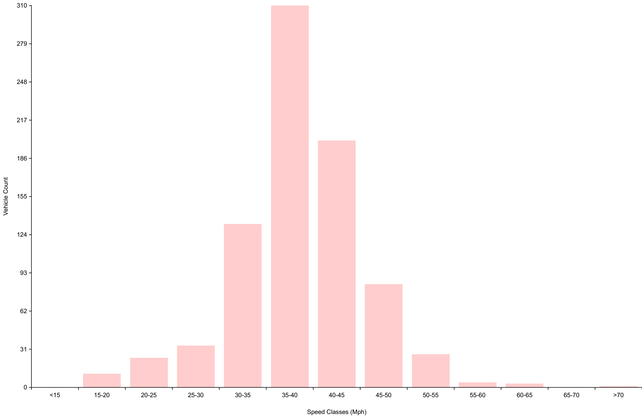
Vehicle Counts By Speed Class For week beginning Mon Aug 3 2026
