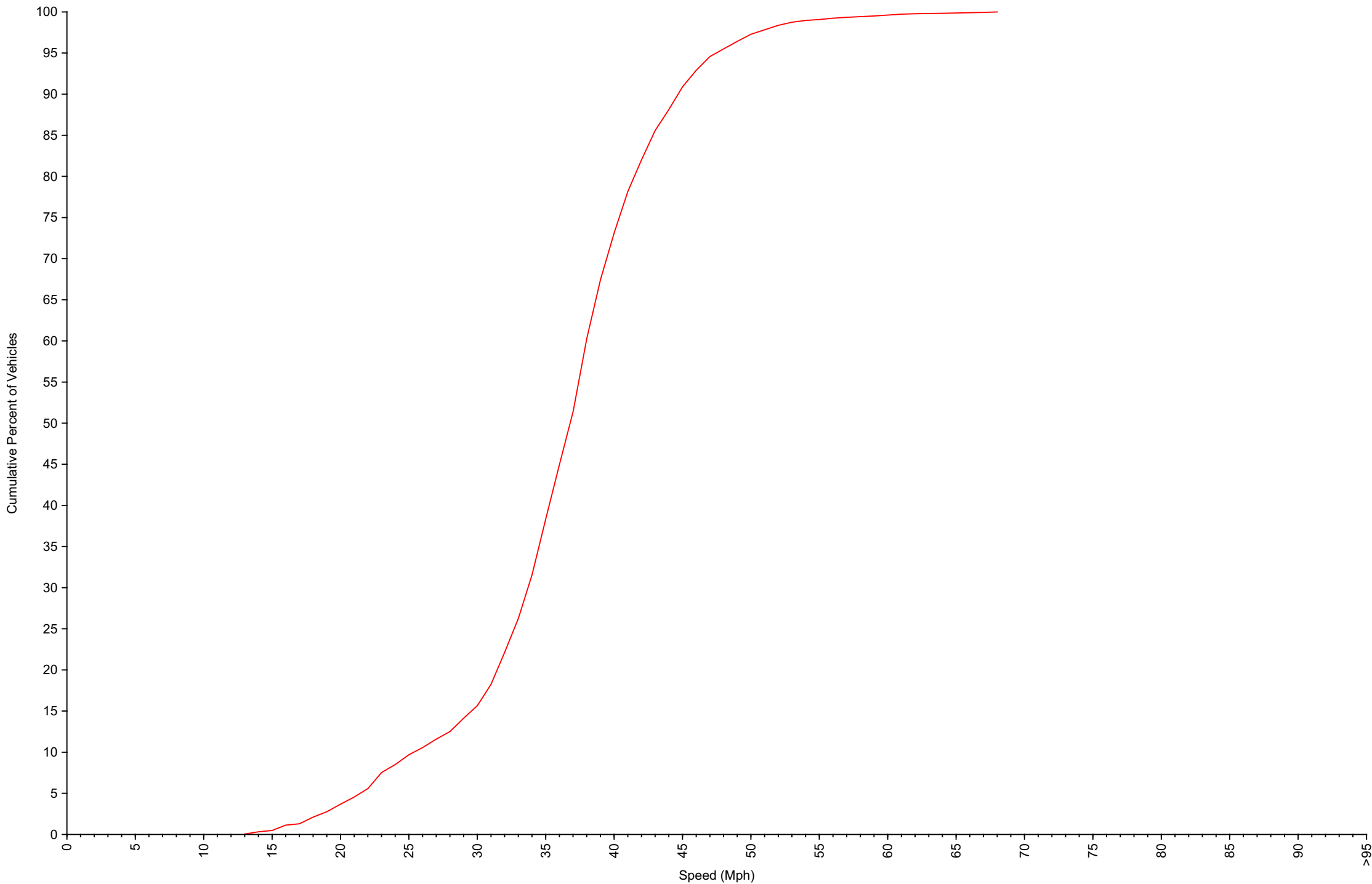
Cumulative Speed Distribution Curve Daily Overview for Sat Aug 15 2026
