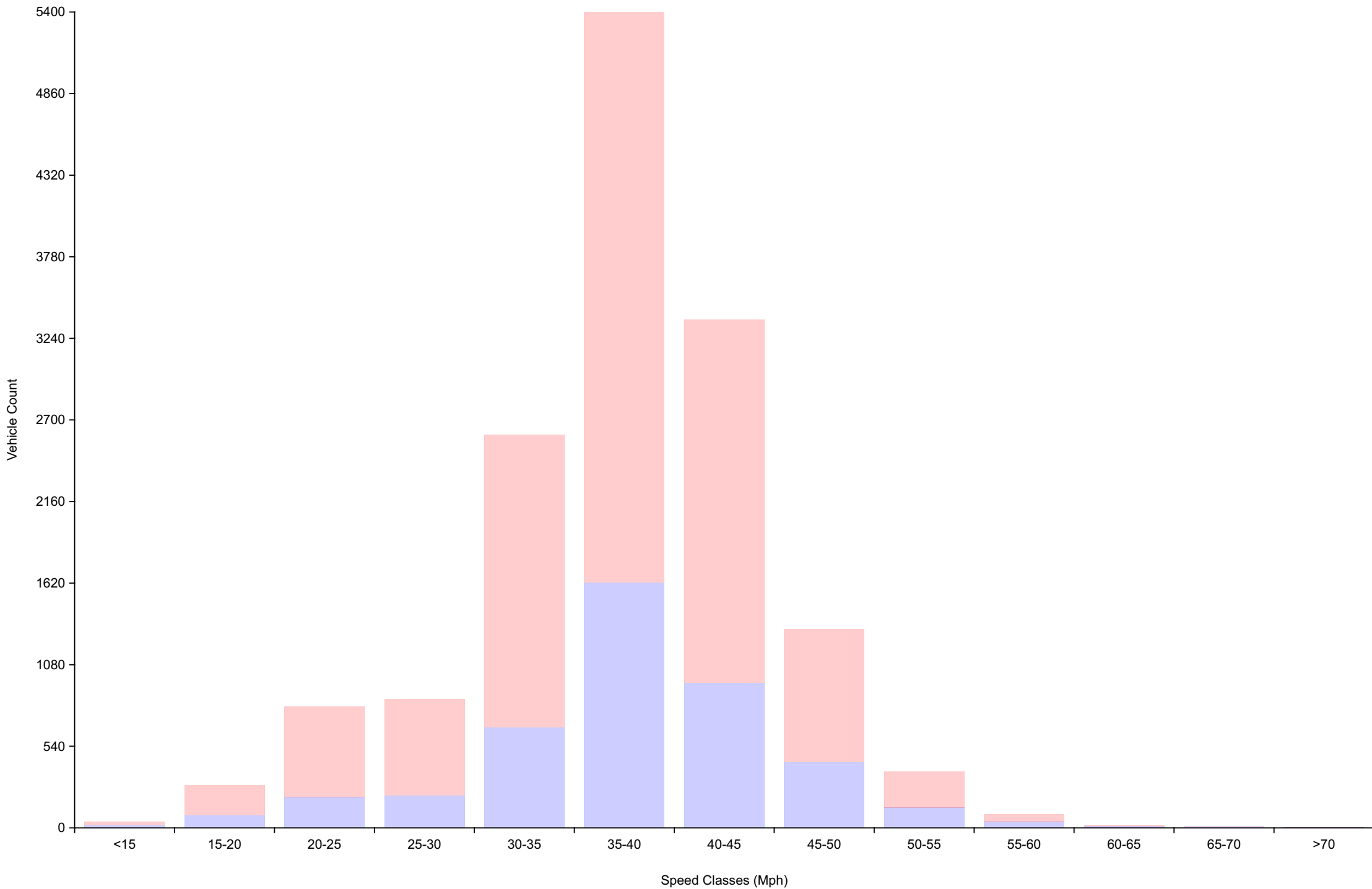
Vehicle Counts By Speed Class For week beginning Mon Aug 10 2026
