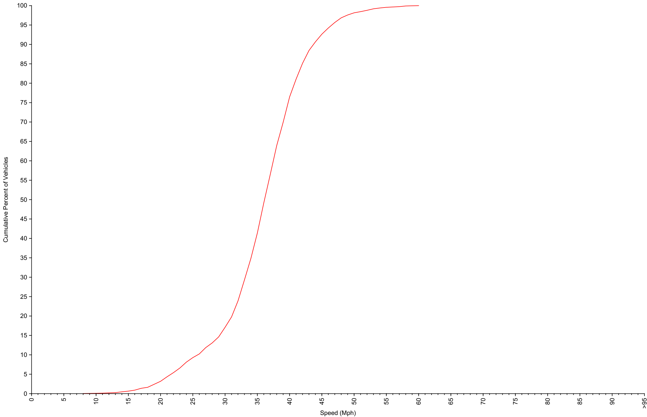
Cumulative Speed Distribution Curve Daily Overview for Mon Aug 24 2026
