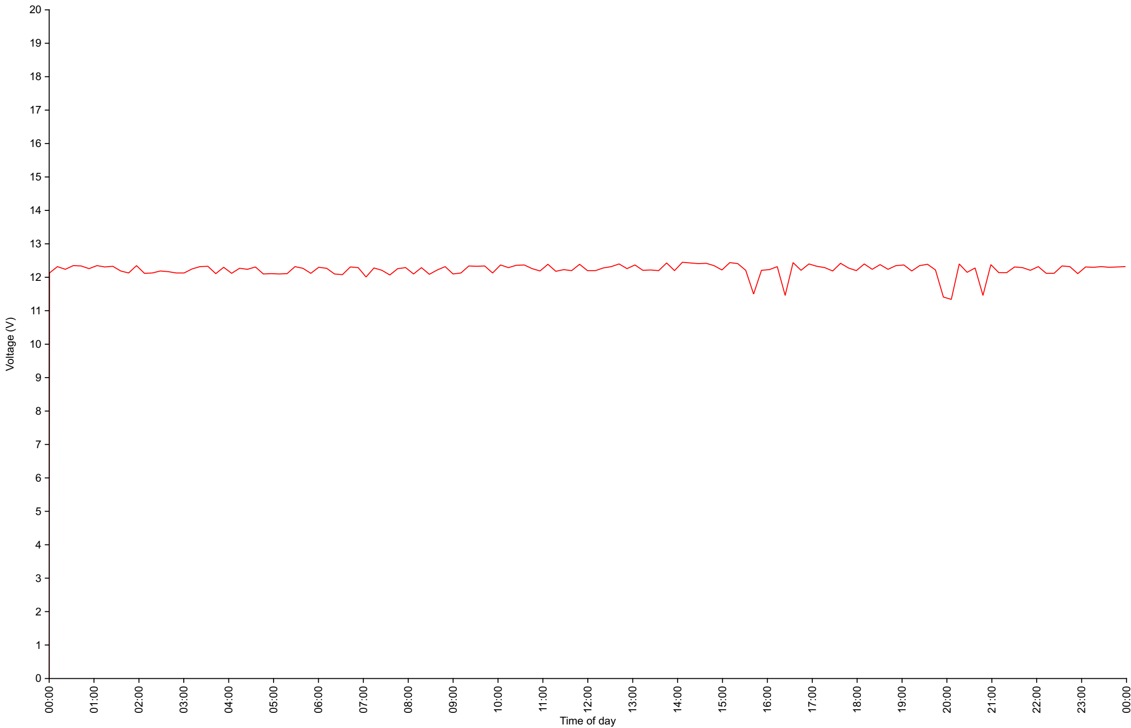
Voltage Daily Overview for Wed Aug 12 2026
