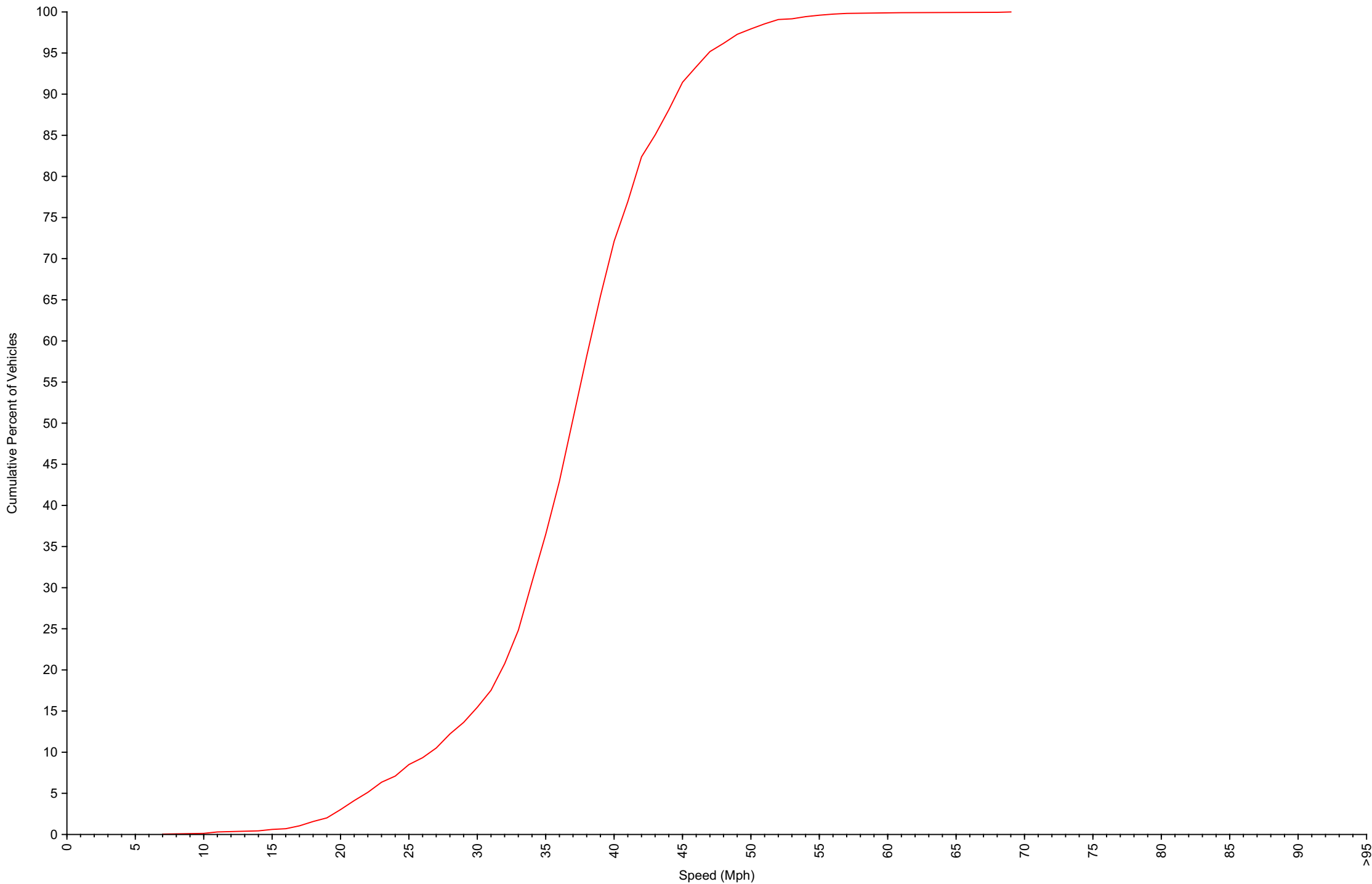
Cumulative Speed Distribution Curve Daily Overview for Tue Aug 11 2026
