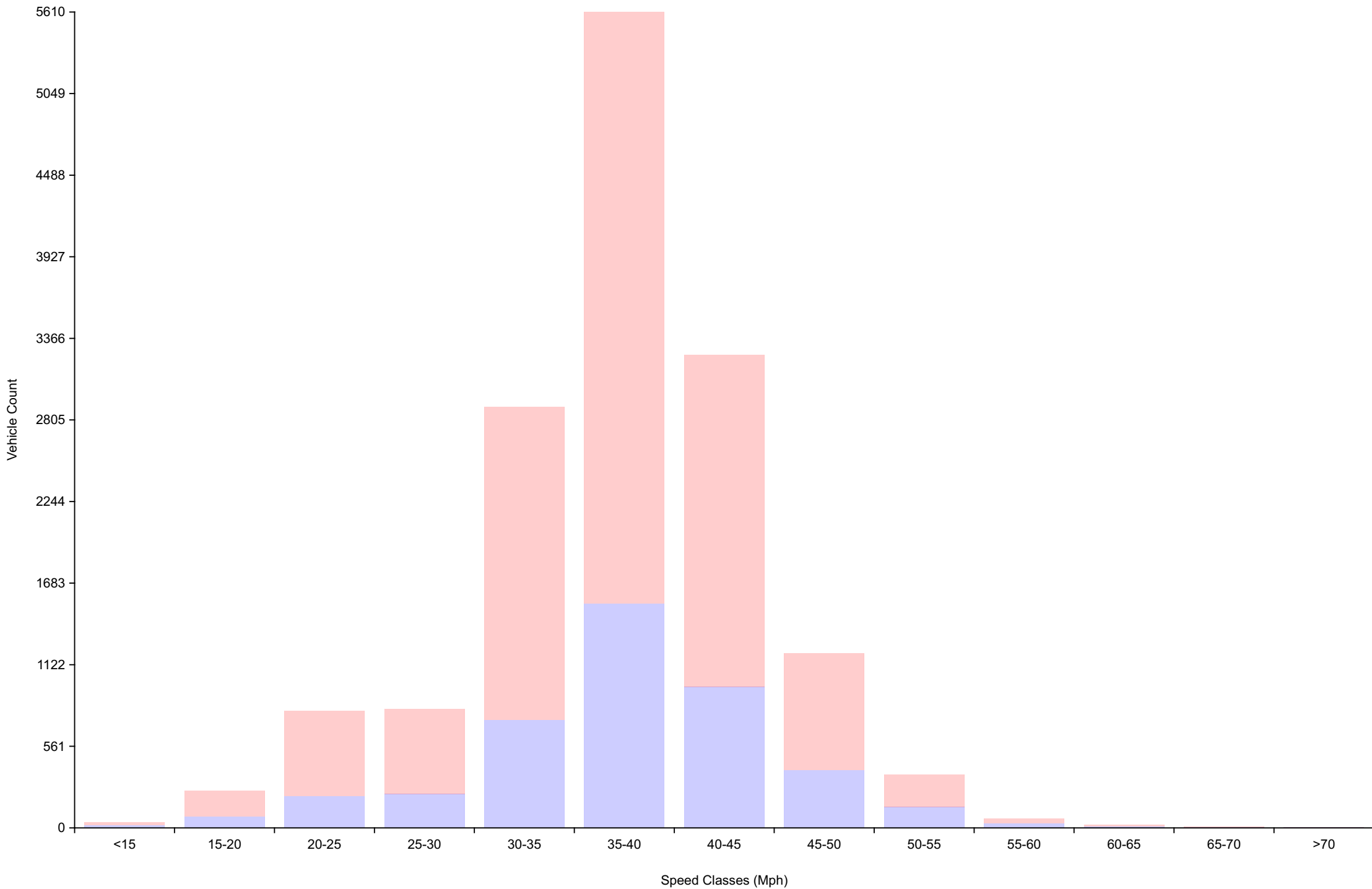
Vehicle Counts By Speed Class For week beginning Mon Aug 17 2026
