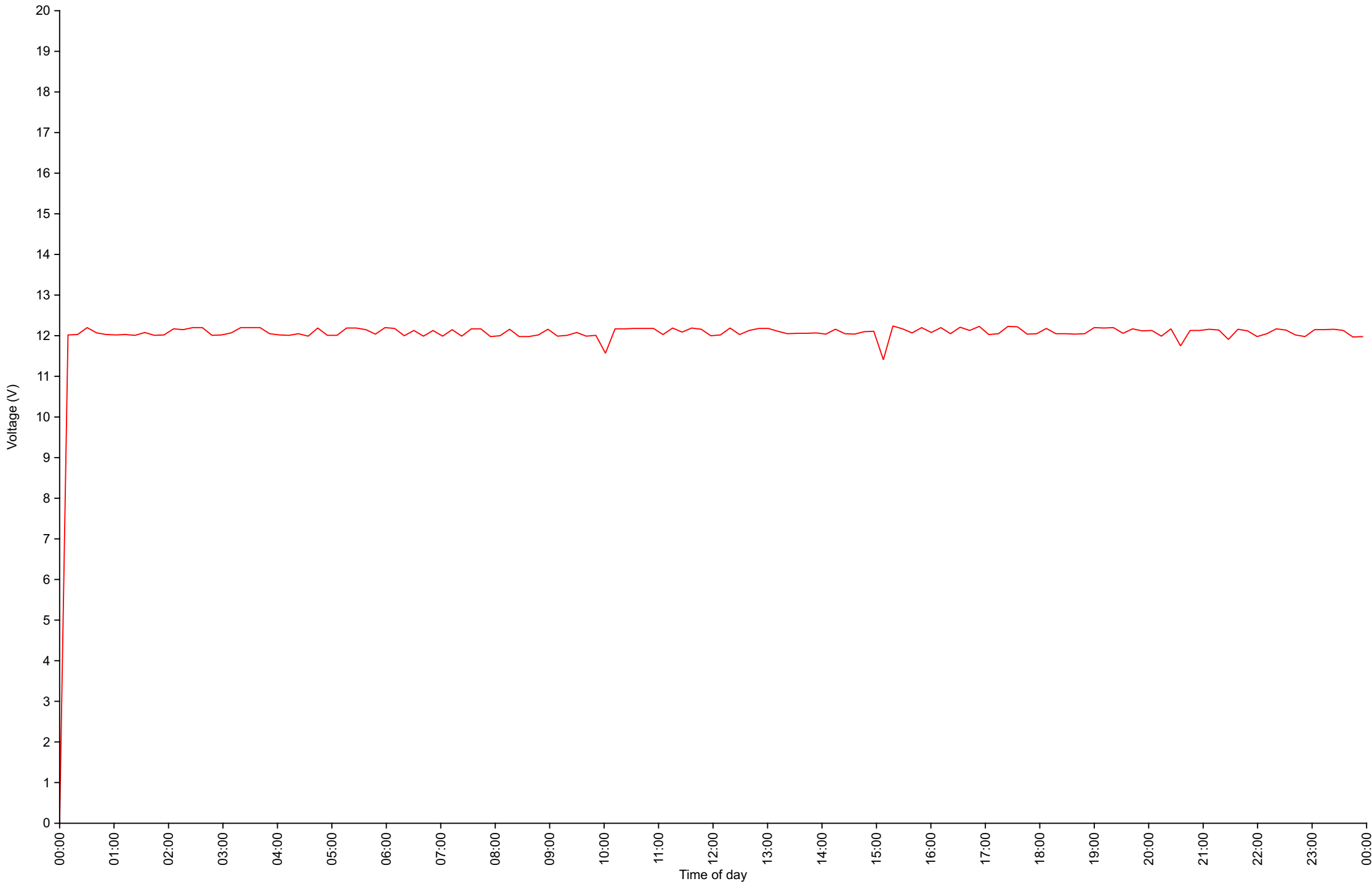
Voltage Daily Overview for Mon Sep 7 2026
