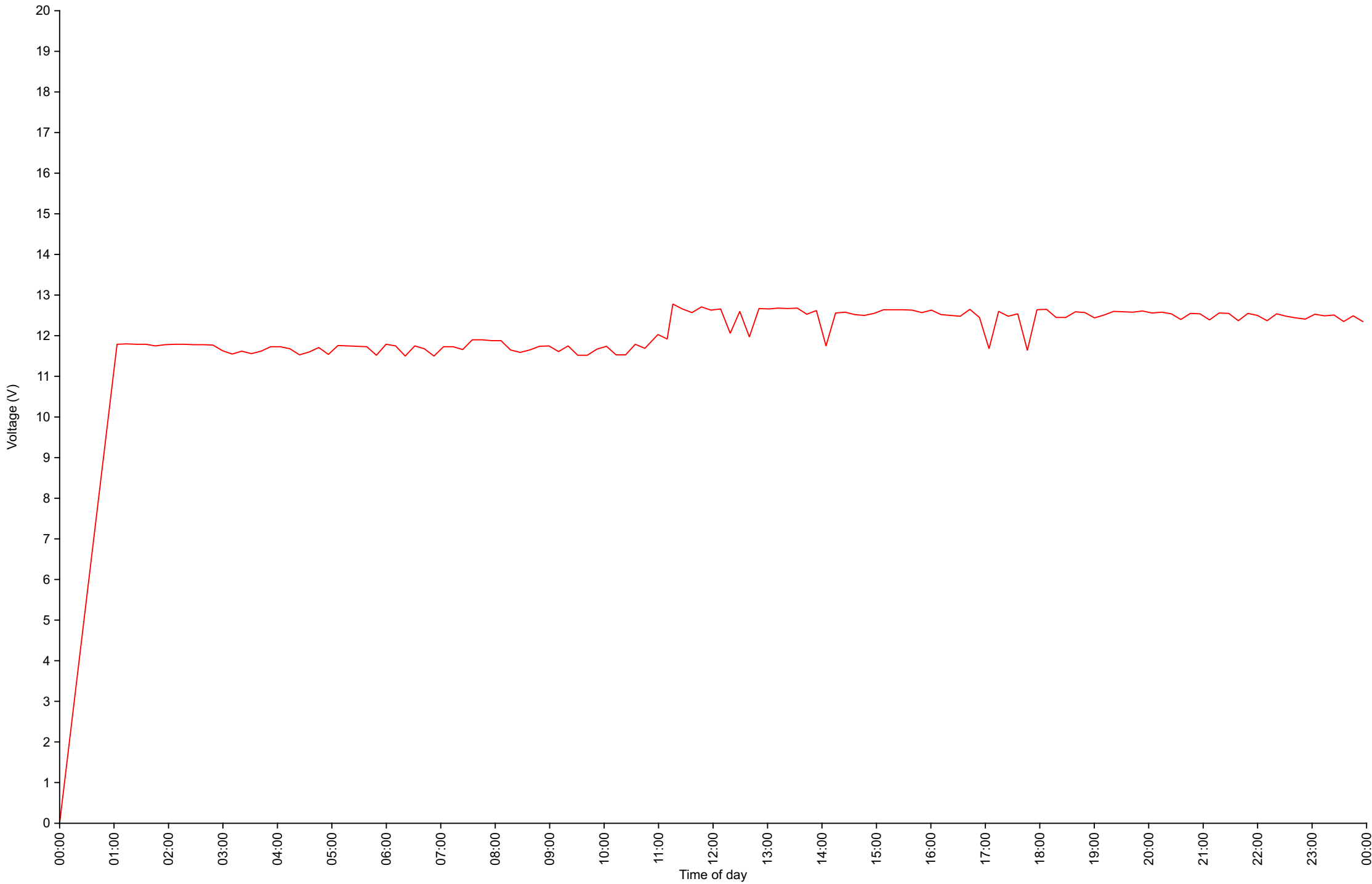
Voltage Daily Overview for Tue Sep 1 2026
