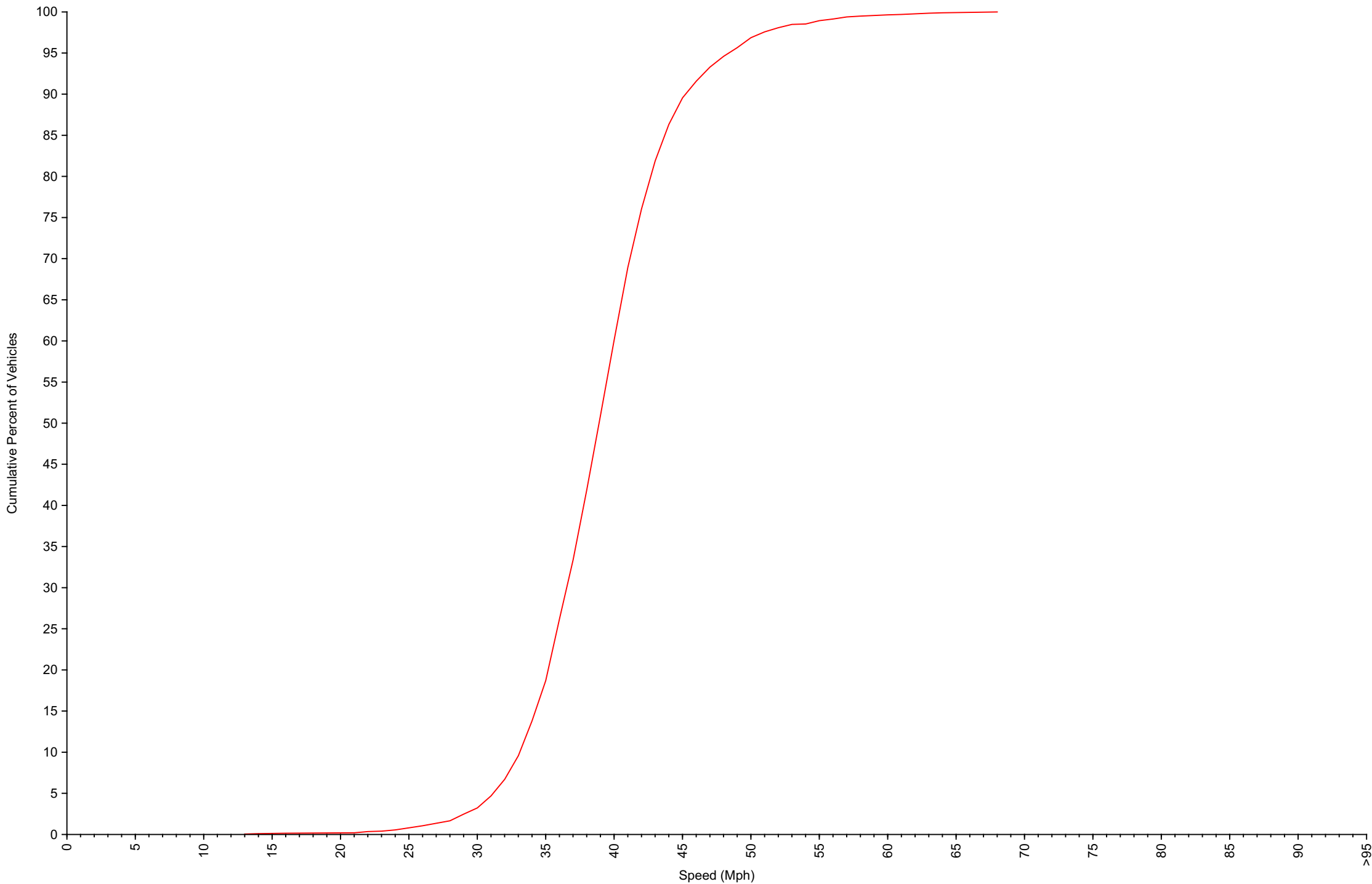
Cumulative Speed Distribution Curve Daily Overview for Thu Sep 10 2026
