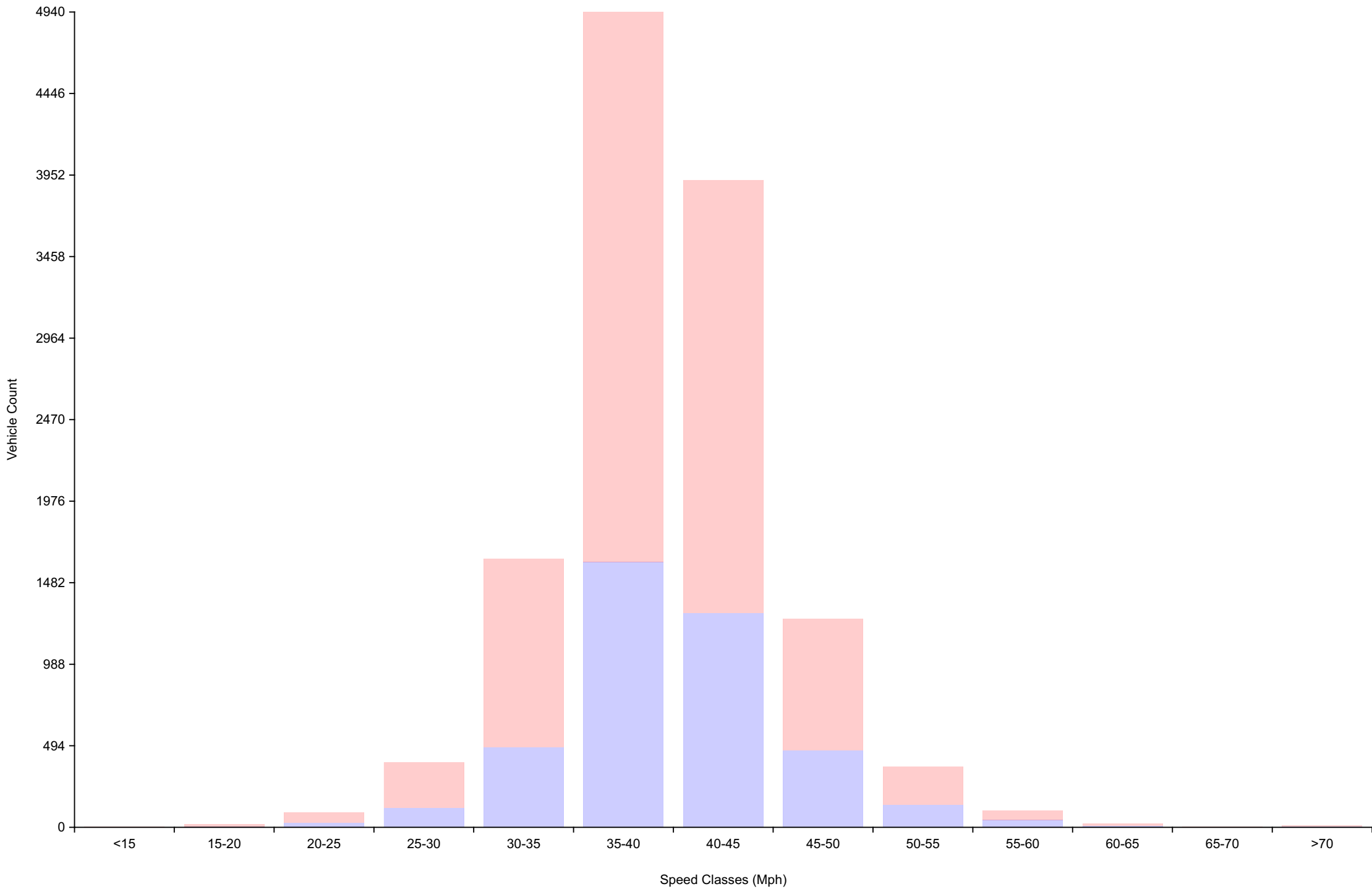
Vehicle Counts By Speed Class For week beginning Mon Aug 31 2026
