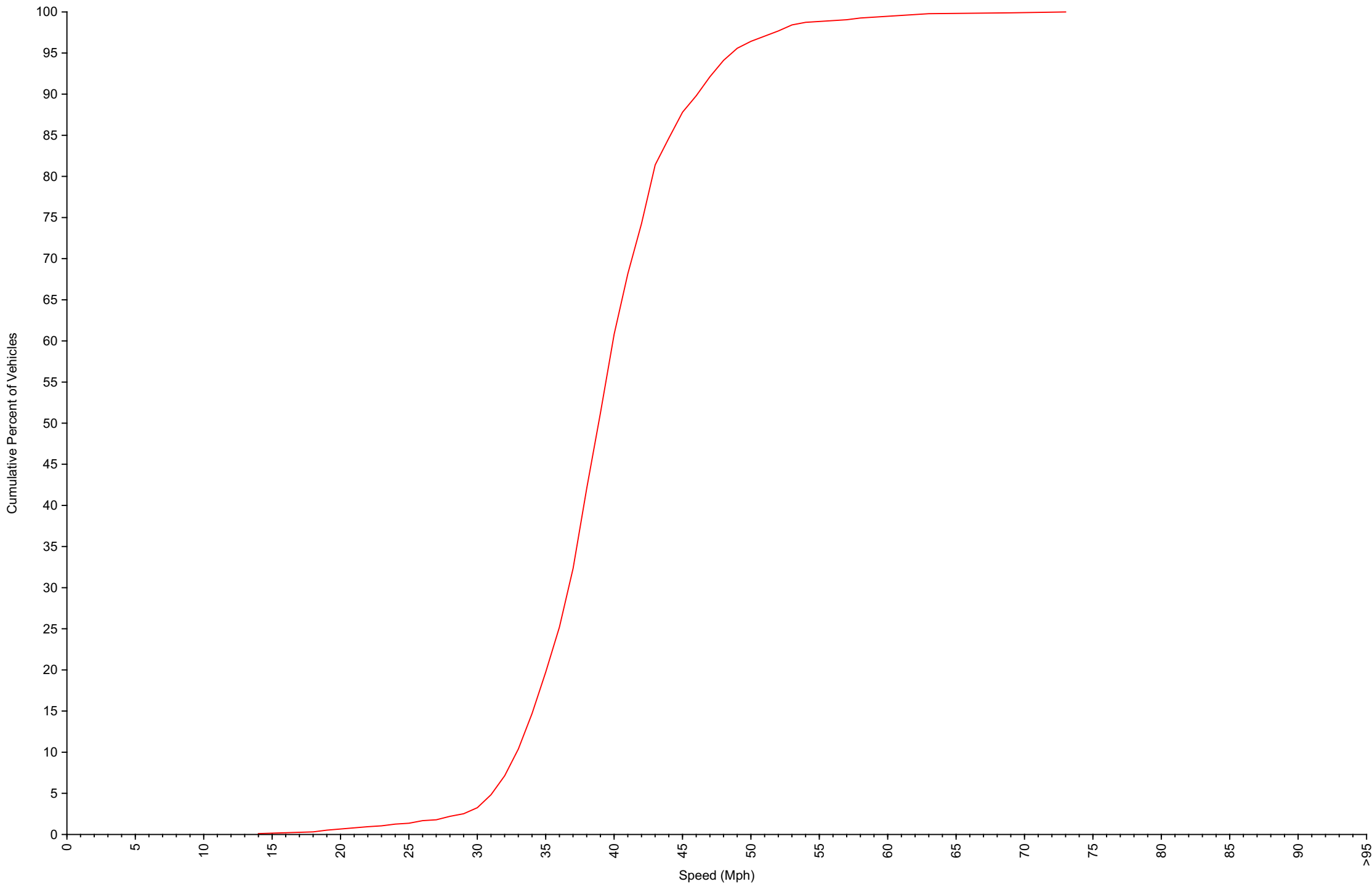
Cumulative Speed Distribution Curve Daily Overview for Sat Sep 19 2026
