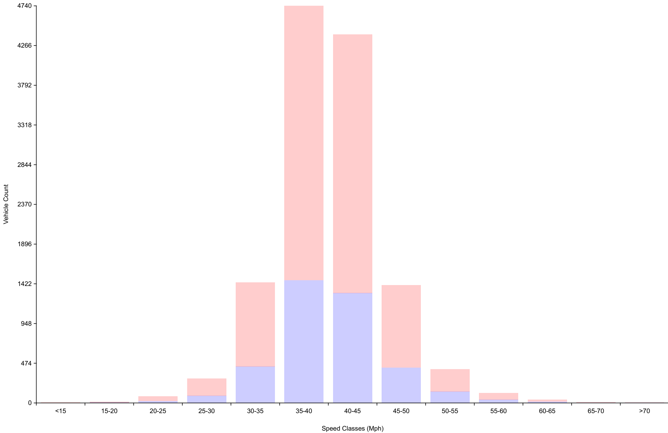
Vehicle Counts By Speed Class For week beginning Mon Sep 7 2026
