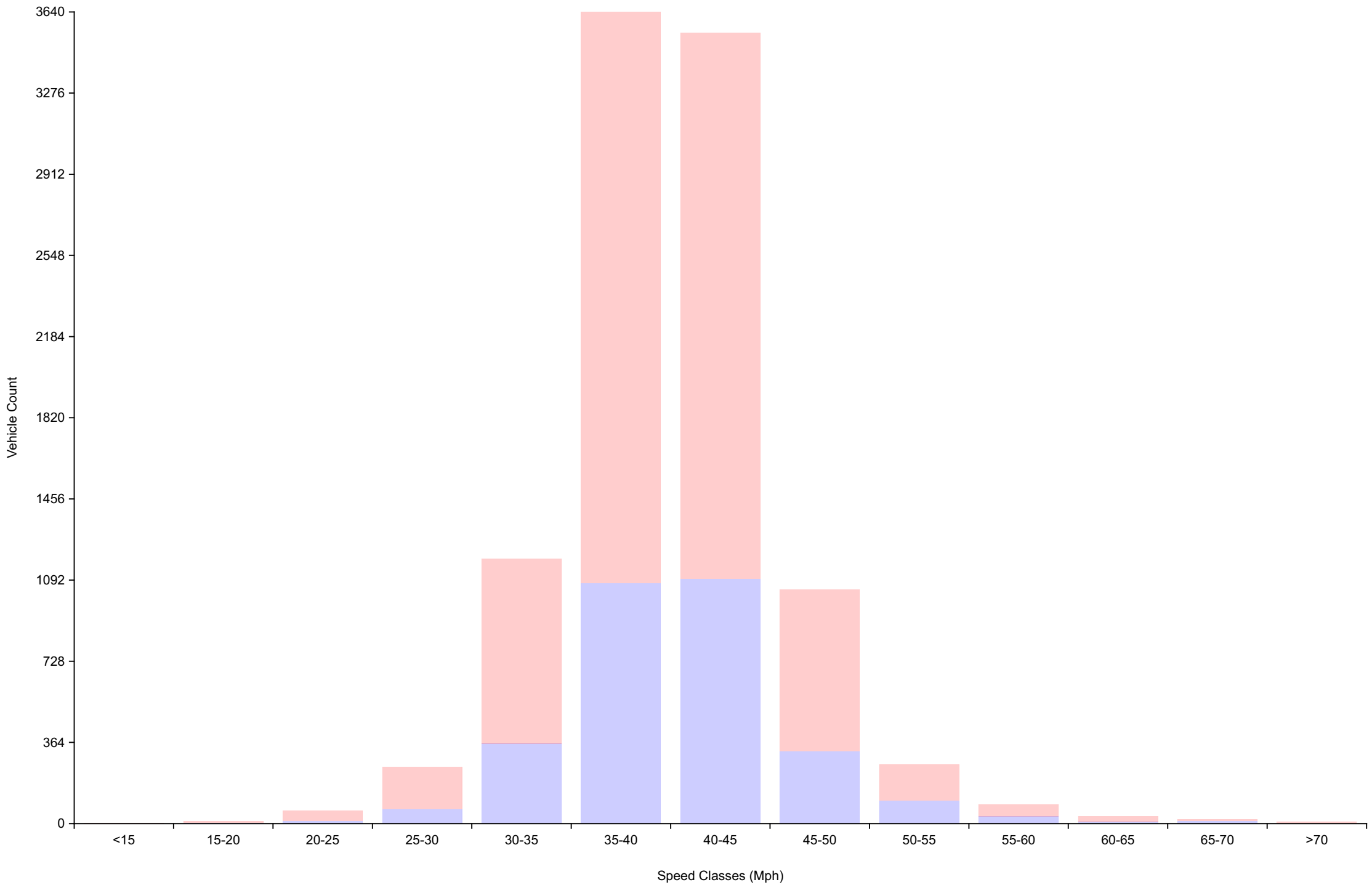
Vehicle Counts By Speed Class For week beginning Mon Sep 14 2026
